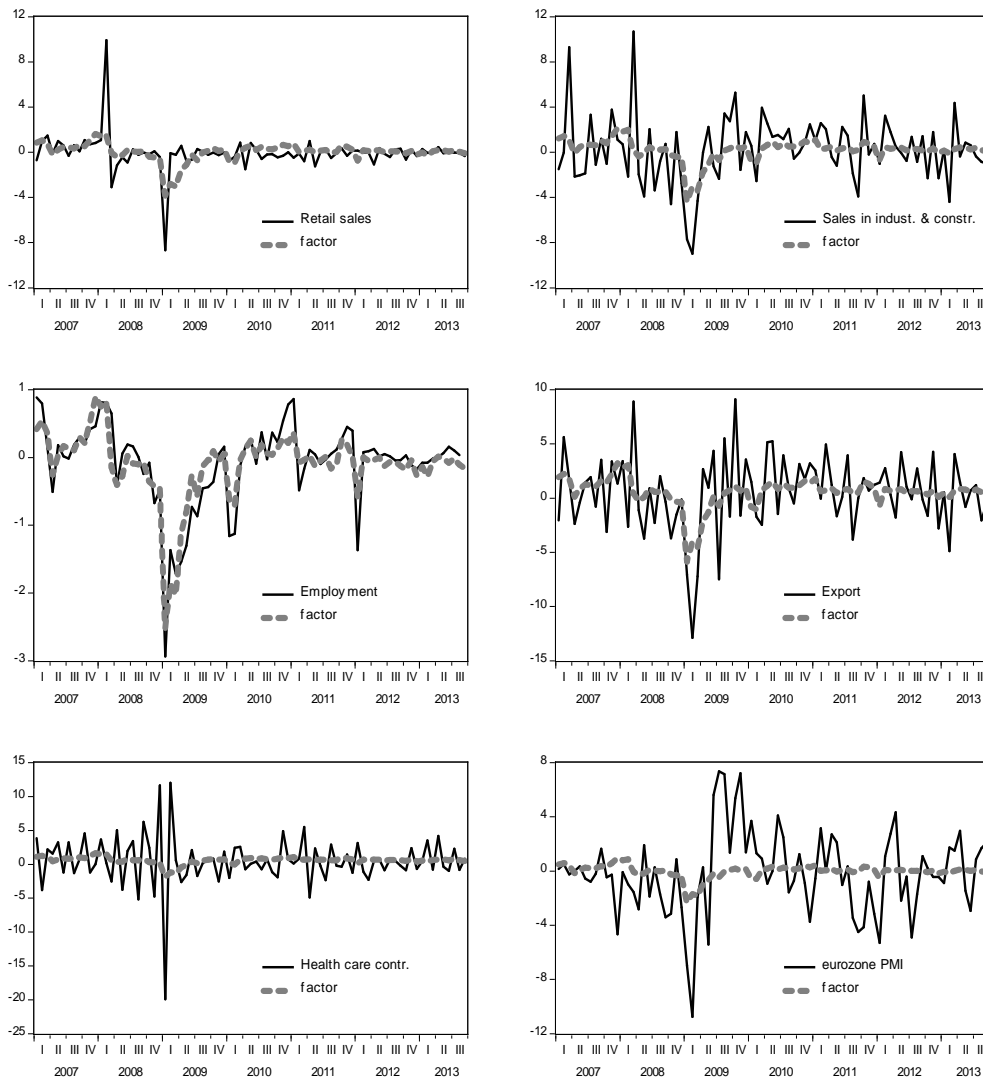
Figure 2 Monthly Indicators and the Common Factor (% m-o-m growth)
